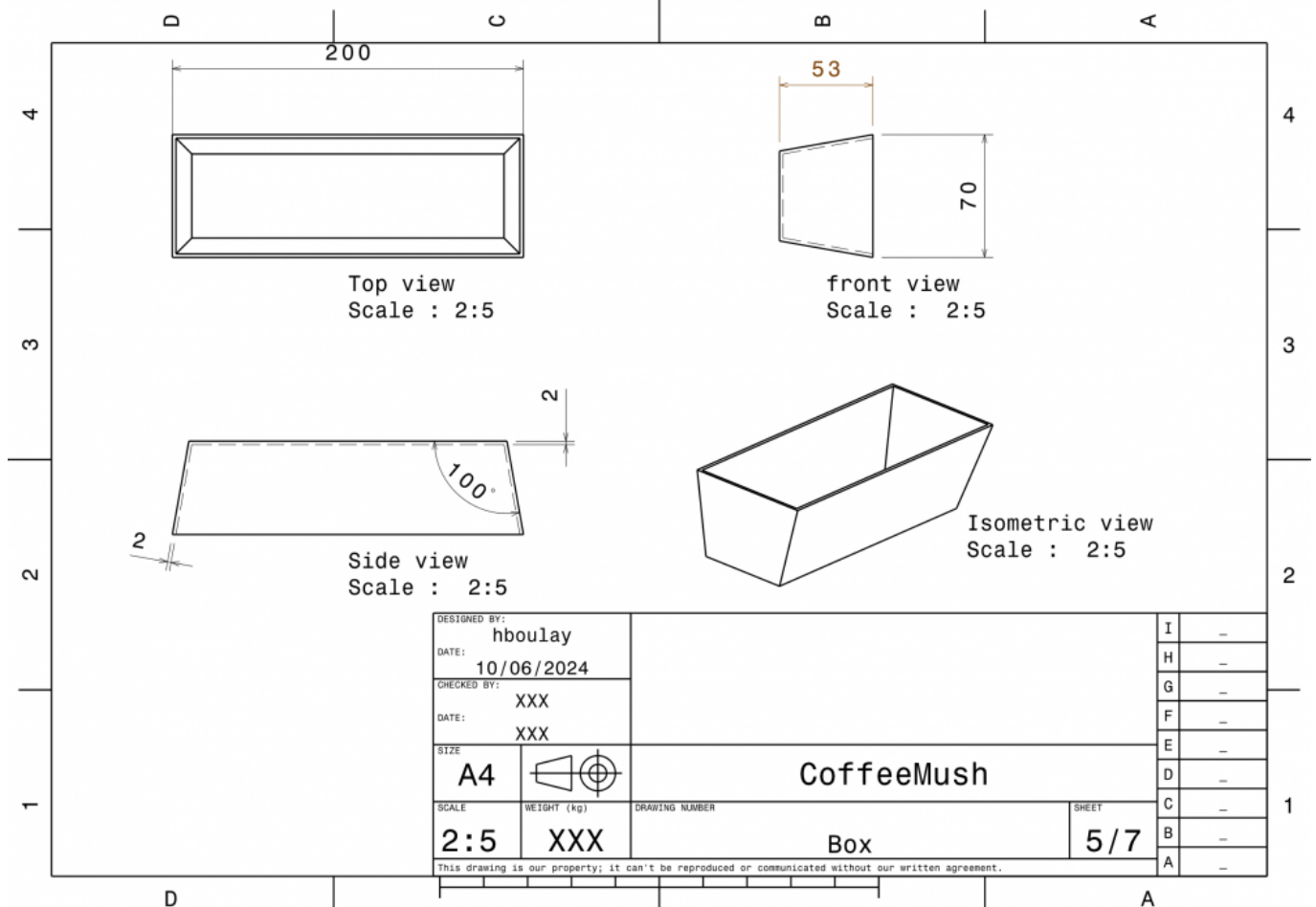
Figure 51: Box
