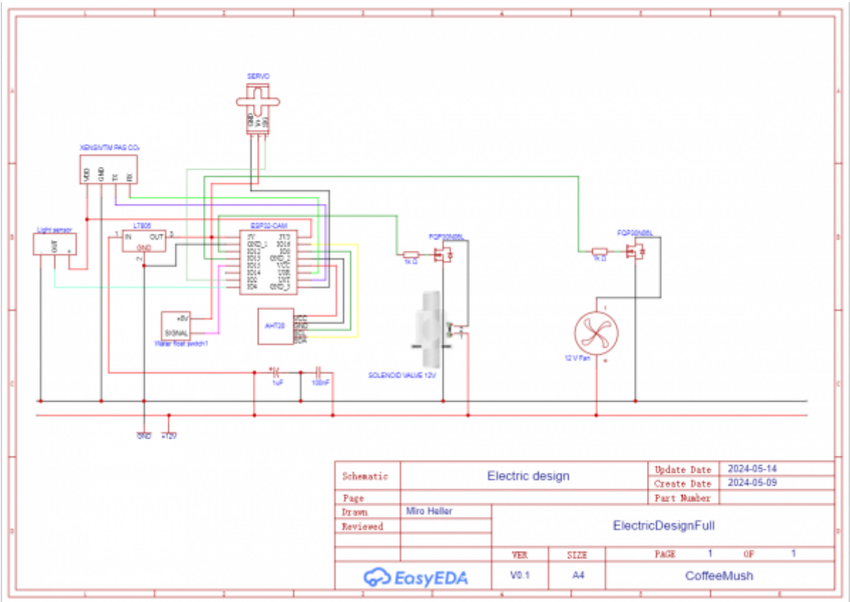
Figure 55: electric schematics
