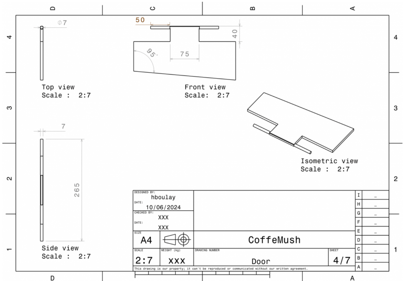
Figure 50: Door
