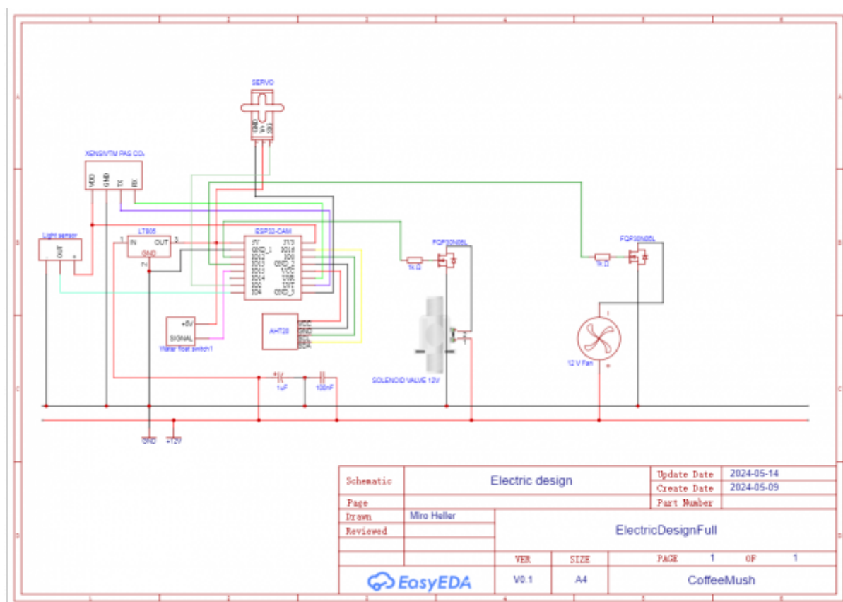
Figure 55: electric schematics
